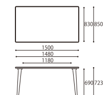
BRIDGE LAMINAM DINING TABLE 150
