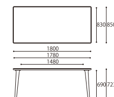
BRIDGE LAMINAM DINING TABLE 180
